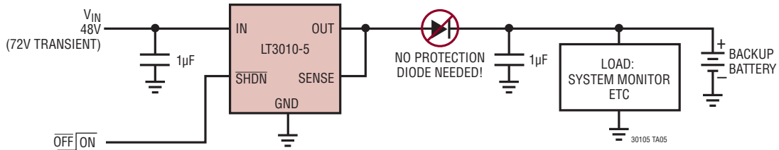
LT3010 Telecom Application
